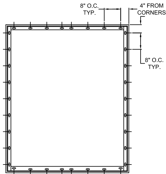
TYPICAL ELEVATION WITH FASTENER SPACING
